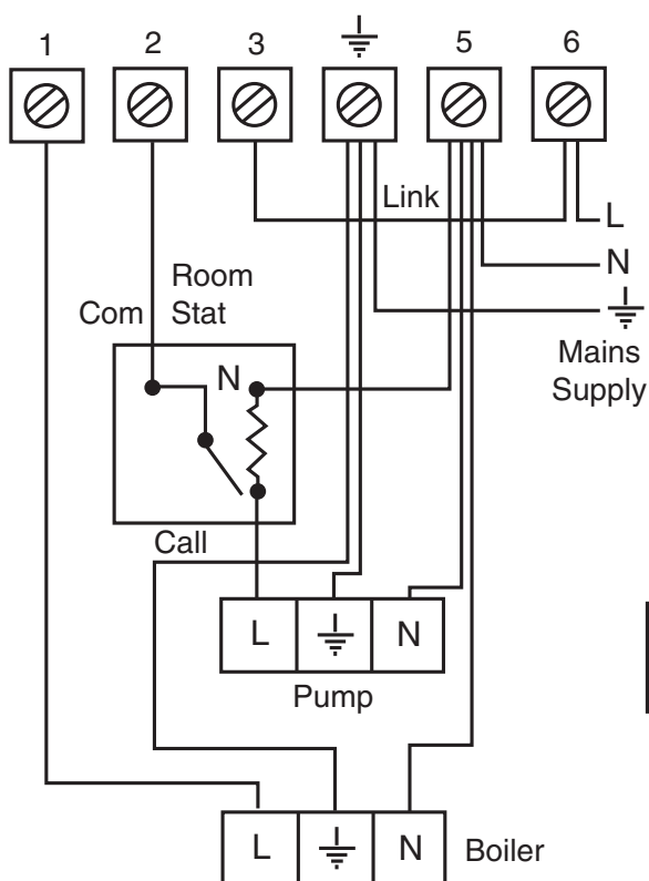
102 Terminals
