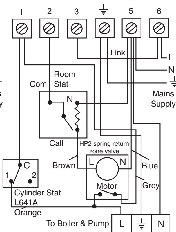
102 Terminals
