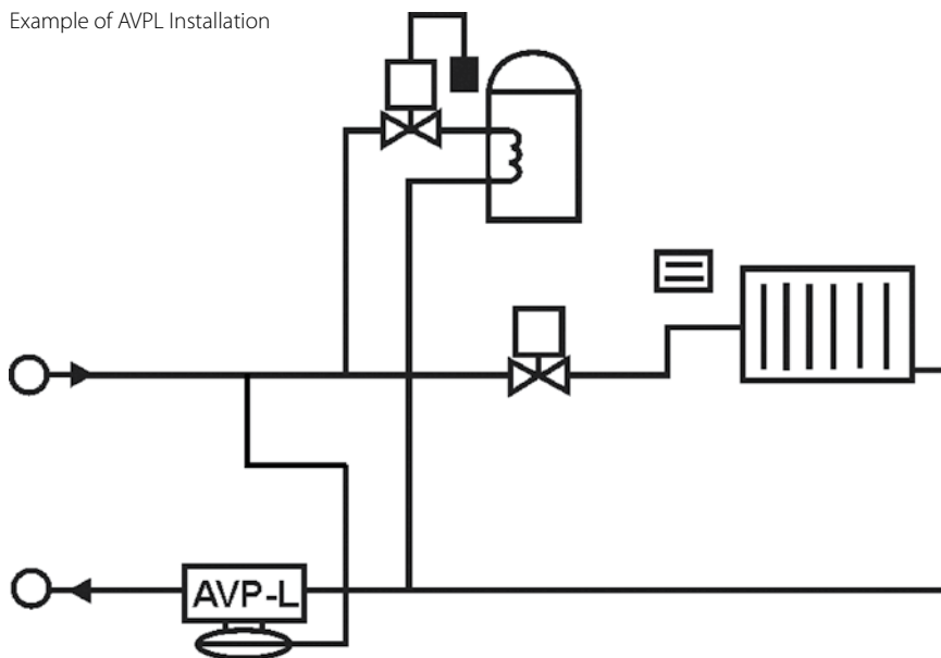
Example of AVPL Installation
